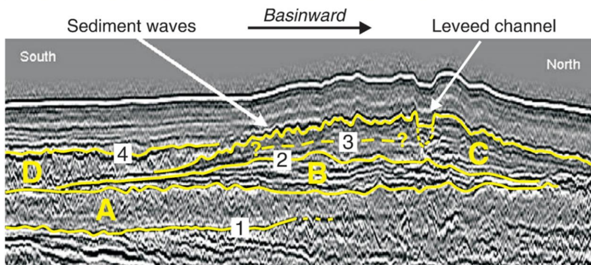
A — mudflow deposits (chaotic internal facies): early stage of forced regression; B — turbidity-flow frontal splay (well-defined parallel reflections): late stage of forced regression; C — leveed channel and overbank facies (high-amplitude reflections associated with the sandy channel fill and weak reflections/transparent facies associated with the finer grained overbank deposits): lowstand normal regressive and early transgressive deposits; D — mudflow deposits (chaotic internal facies): late transgressive deposits. Note the gradual progradation of gravity-flow deposits into the basin from A to C, and the retrogradation from C to D. Sequence stratigraphic surfaces: 1 — correlative conformity sensu Posamentier and Allen (1999) ; 2 — correlative conformity sensu Hunt and Tucker (1992) ; 3 — maximum regressive surface (cryptic, within an undifferentiated succession of low-density leveed-channel turbidites); and 4 — maximum flooding surface.
