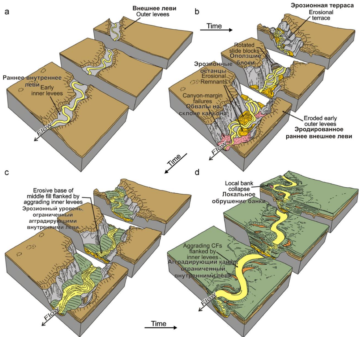
Schematic block diagrams illustrating the evolution of the Benin-major Canyon and its fill. (a) Early incision of the canyon, with deposition of outer levees, perhaps with contemporaneous deposition of early inner levees. (b) Over-deepening of the canyon, with prominent erosion of outer levee crests and eventual scavenging of early fill deposits during periods of re-incision and canyon flushing. (c) Final erosion at base of middle fill associated with laterally migrating channels flanked by aggradational inner levees that drape elevated interchannel areas. (d) Predominantly aggradational channel deposits flanked by aggradational inner levees that form the most important fill of the Benin-major Canyon (in terms of volume). Aggradation of these deposits progressively smooths over the underlying canyon morphology, though it still has an expression at the seafloor.
